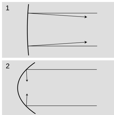
e/ Mirror 1 is weaker than mirror 2. It has a shallower curvature, a longer focal length, and a smaller focal angle. It reflects rays at angles not much different than those that would be produced with a flat mirror.
